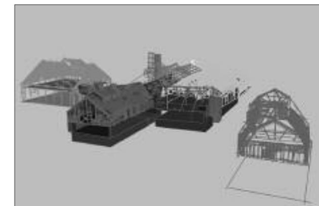
Wire-frame model of the Lion Salt Works produced from a laser scan survey funded by English Heritage.
